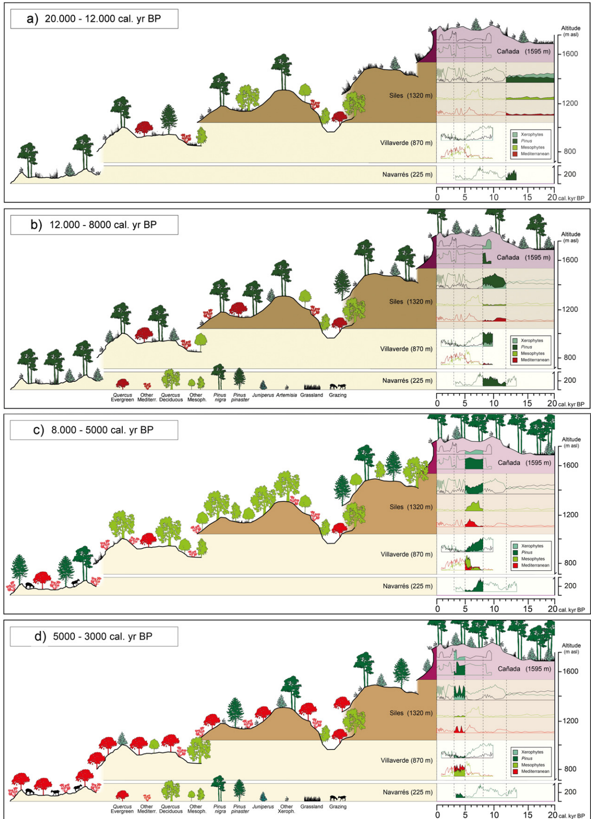
Fig. 3. Altitudinal vegetation dynamics in the Segura Mountains (SE Iberia) for the last 20,000 years ago: (a) Late Pleniglacial and Late Glacial, (b) Late Pleistocene and Early Holocene, (c) Holocene Mesophytic Optimum, and (d) Mid-Holocene. Based on Carrión (2002b).
